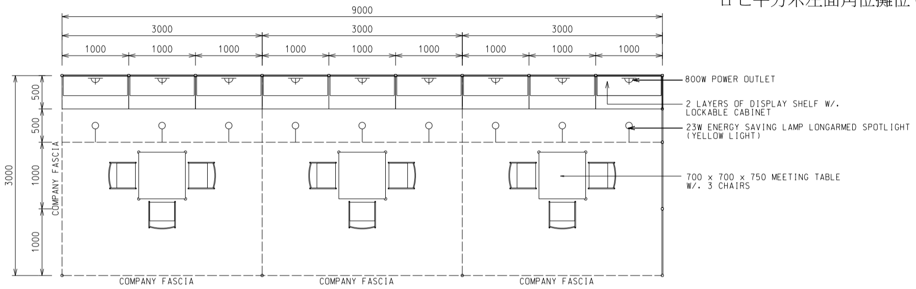
PLAN 9M(W) X 3M(D) X 2.5M(H) Left Corner Booth A
