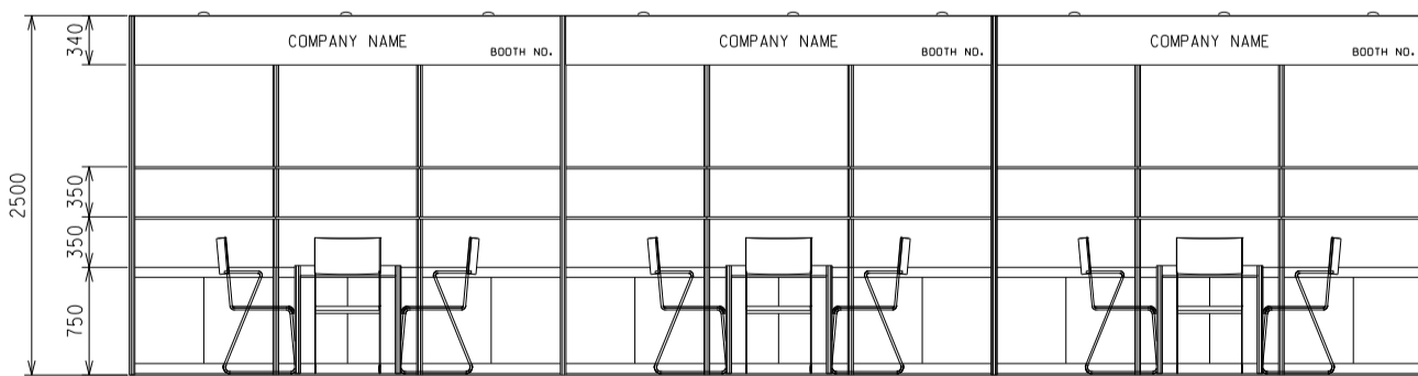
ELEVATION 9M(W) X 3M(D) X 2.5M(H) Left Corner Booth A
